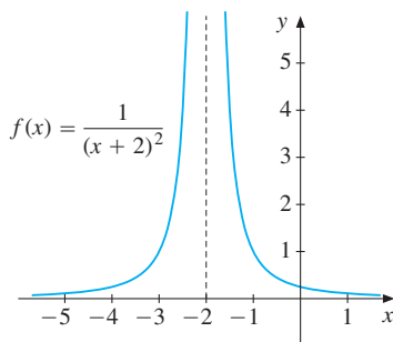
Figure 1 f(x) \rightarrow \infty as x \rightarrow -2
