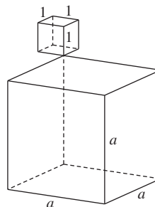
Figure 2 Volume a^3 + 1
