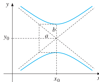
Figure 7 Hyperbola
