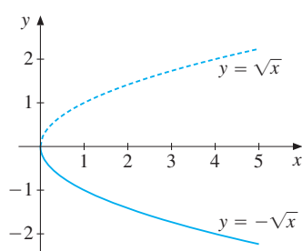
Figure 4 y = \pm\sqrt{x}
