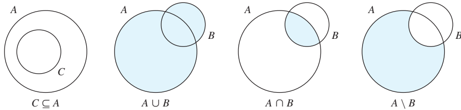
Figure 1 Venn diagrams
