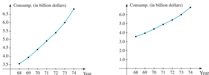
Figure 6 Graphical representations of the same function with different units of measurement
