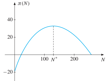
Figure 2 Profit function in Example 1(b)
