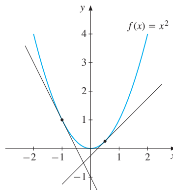
Figure 5 f(x) = x^2
