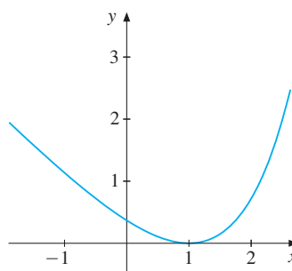
Figure 4 f(x) = e^{x-1} - x
