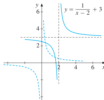
Figure 7 y = 1/(x - 2) + 3
