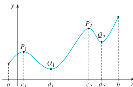
Figure 1 c_1 , c_2 , and b are local maximum points; a , d_1 , and d_2 are local minimum points
