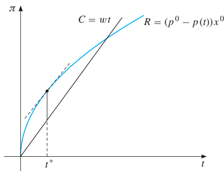
Figure 1 Optimal search
