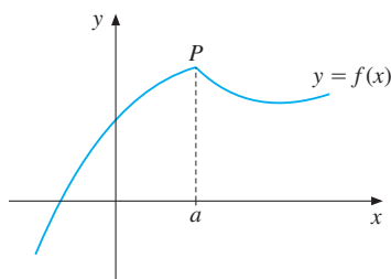
Figure 1 A continuous function
