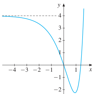
Figure 3 f(x) = e^{2x} - 5e^x + 4
