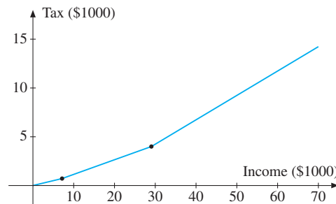
Figure 8 US Federal Income Tax in 2004
