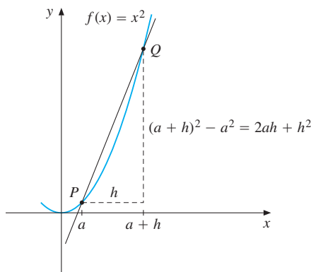
Figure 4 f(x) = x^2
