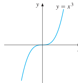
Figure 4 f'(0) = f''(0) = 0 , and 0 is an inflection point
