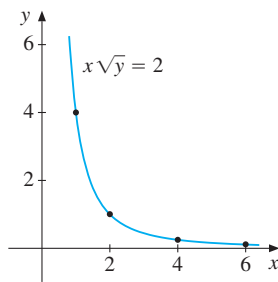
Figure 1 x\sqrt{y} = 2
