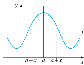
Figure 6 Symmetric about x = a
