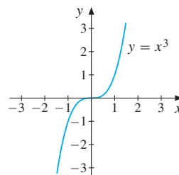
Figure 7 y = x^3
