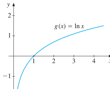
Figure 1 The graph of the logarithmic function g(x) = \ln x
